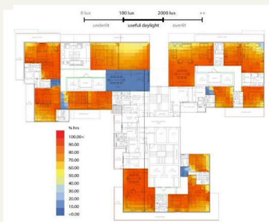
Figure 4.1 UDI Analysis with a Daylighting Analysis Software
